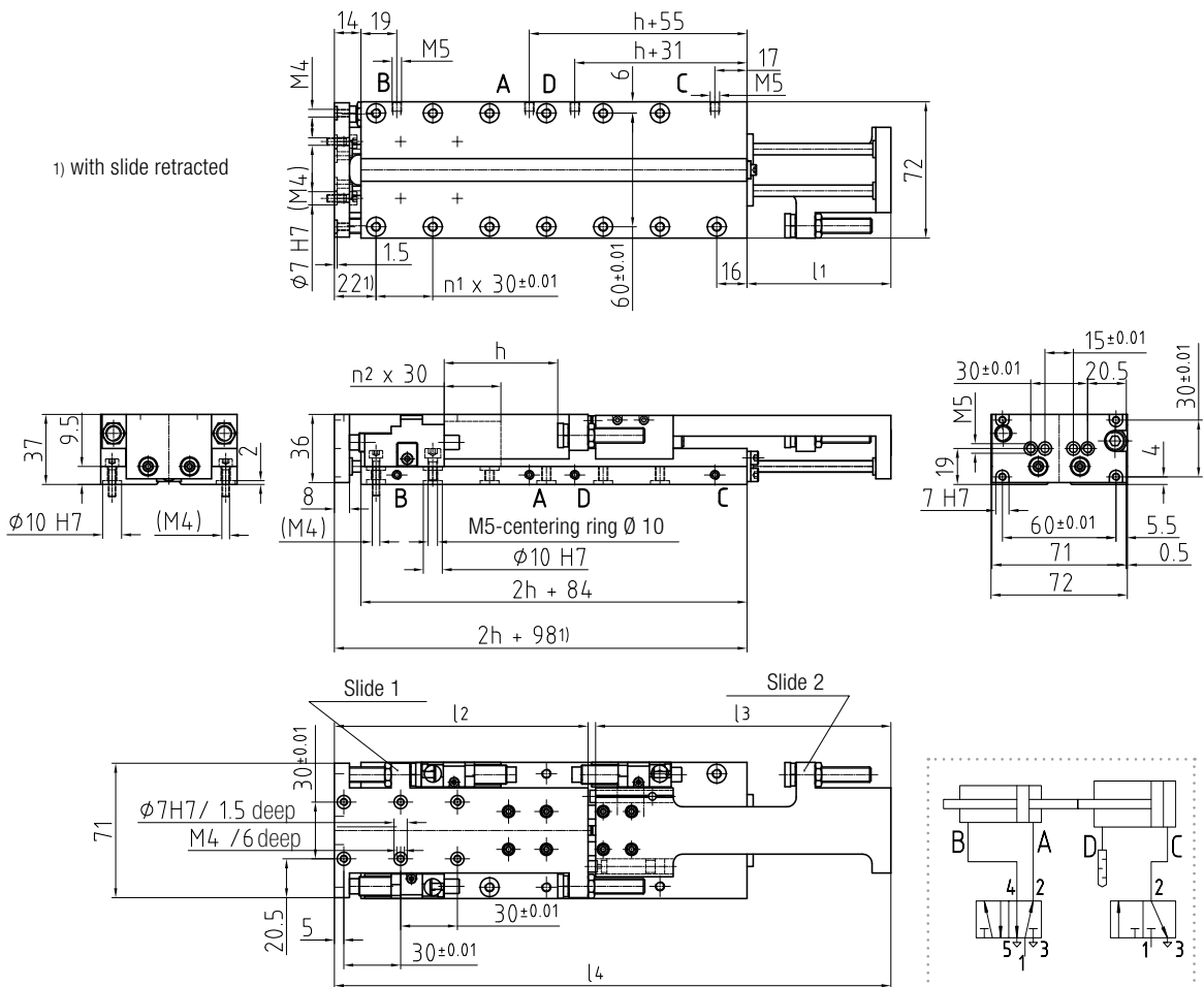
Dimensional drawing and pneumatic diagram
