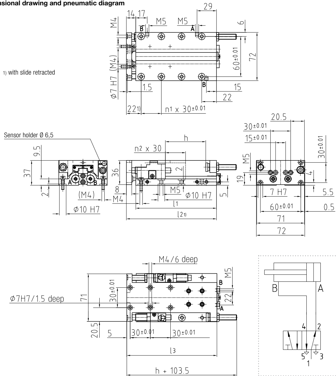
Dimensional drawing and pneumatic diagram
