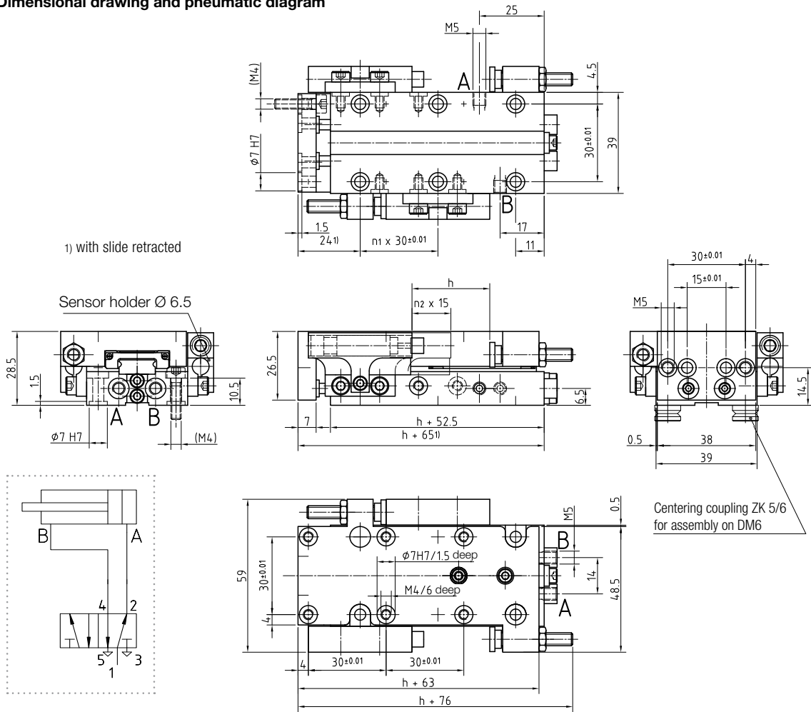
Dimensional drawing and pneumatic diagram
